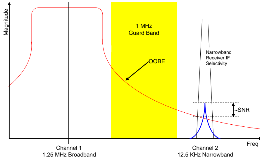
Figure 2 – Source of interference due to OBE
