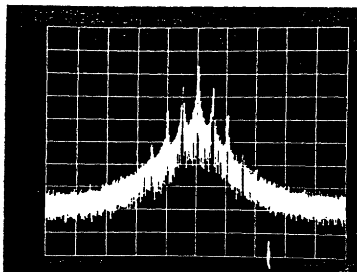
Figure 4 Mode GT2A emission from LANDSAT-D.
