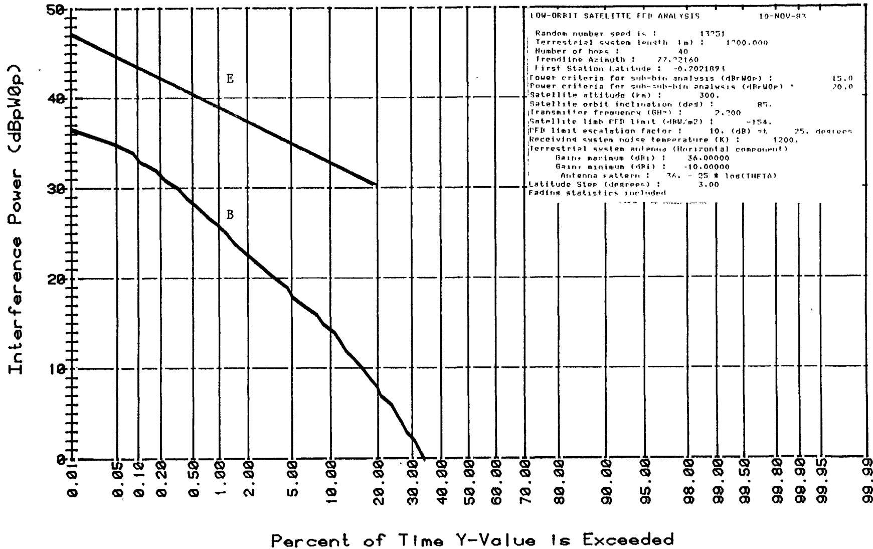
Figure 29 Interference Power From Eight Satellites in Non-Geostationary Orbits to Radio-Relay Receivers in a Trendline Using Single Frequency Plan.
