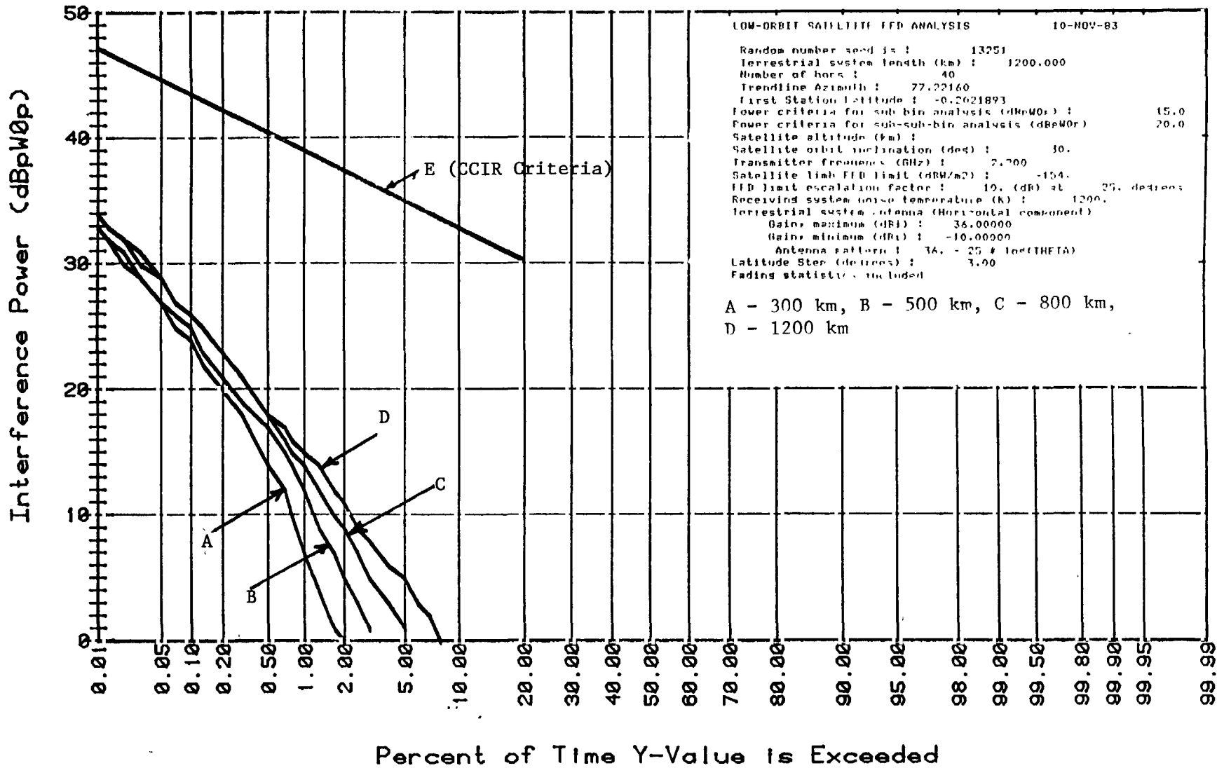
Figure 13 Interference Calculation for Inclination Angle Equal to 10 Degrees
