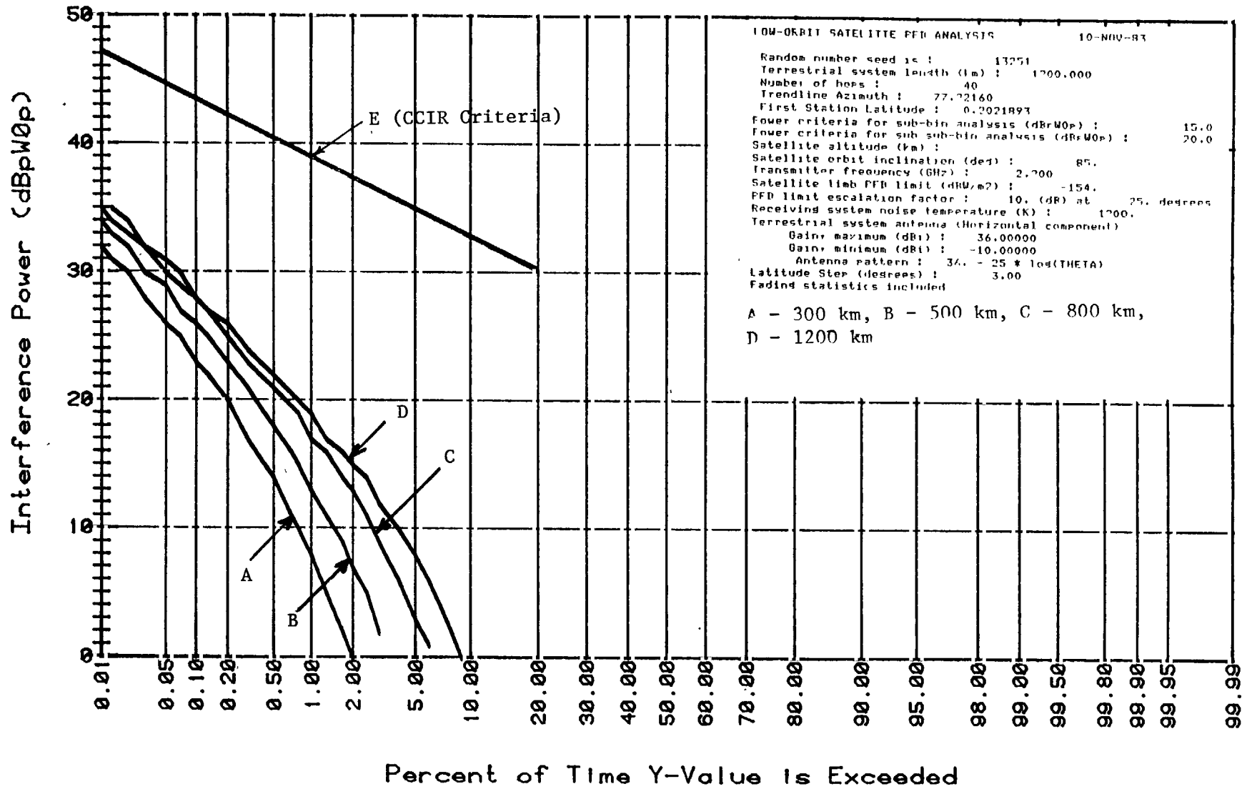
Figure 16 Interference Calculations for Inclination Angle Equal to 85 Degrees
