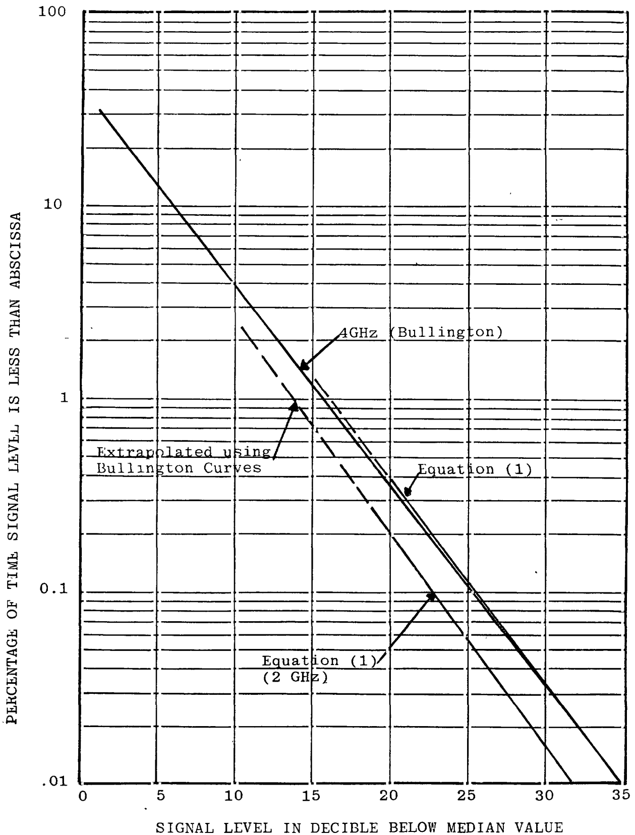
FIGURE 10: Comparison of Bullington results with data given by Equation (1)
