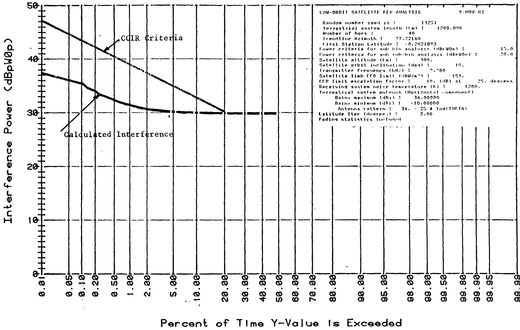
FIGURE 17: Combined Interference from Satellites in Both Geostationary and Non-Geostationary Orbits
