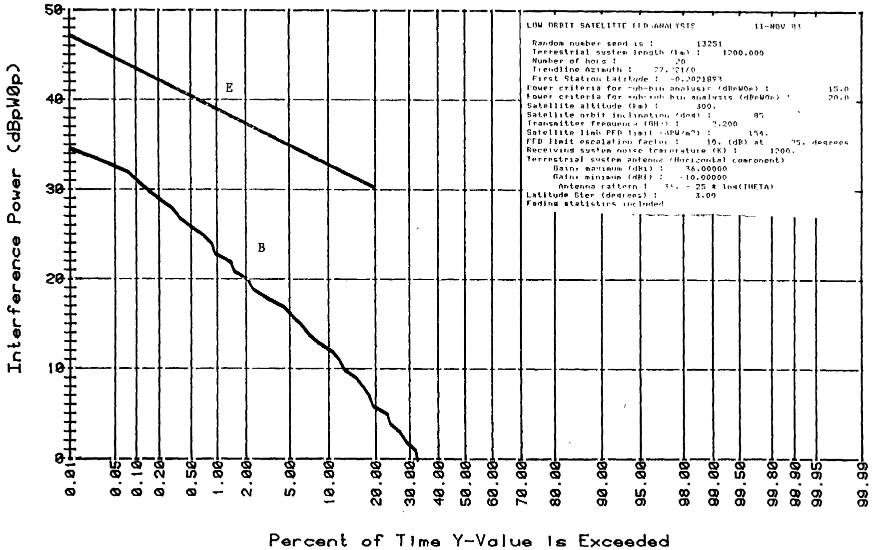
Figure 30 Interference Power From Eight Satellites in Non-Geostationary Orbits to Radio-Relay Receivers in a Trendline Using Double Frequency Plan
