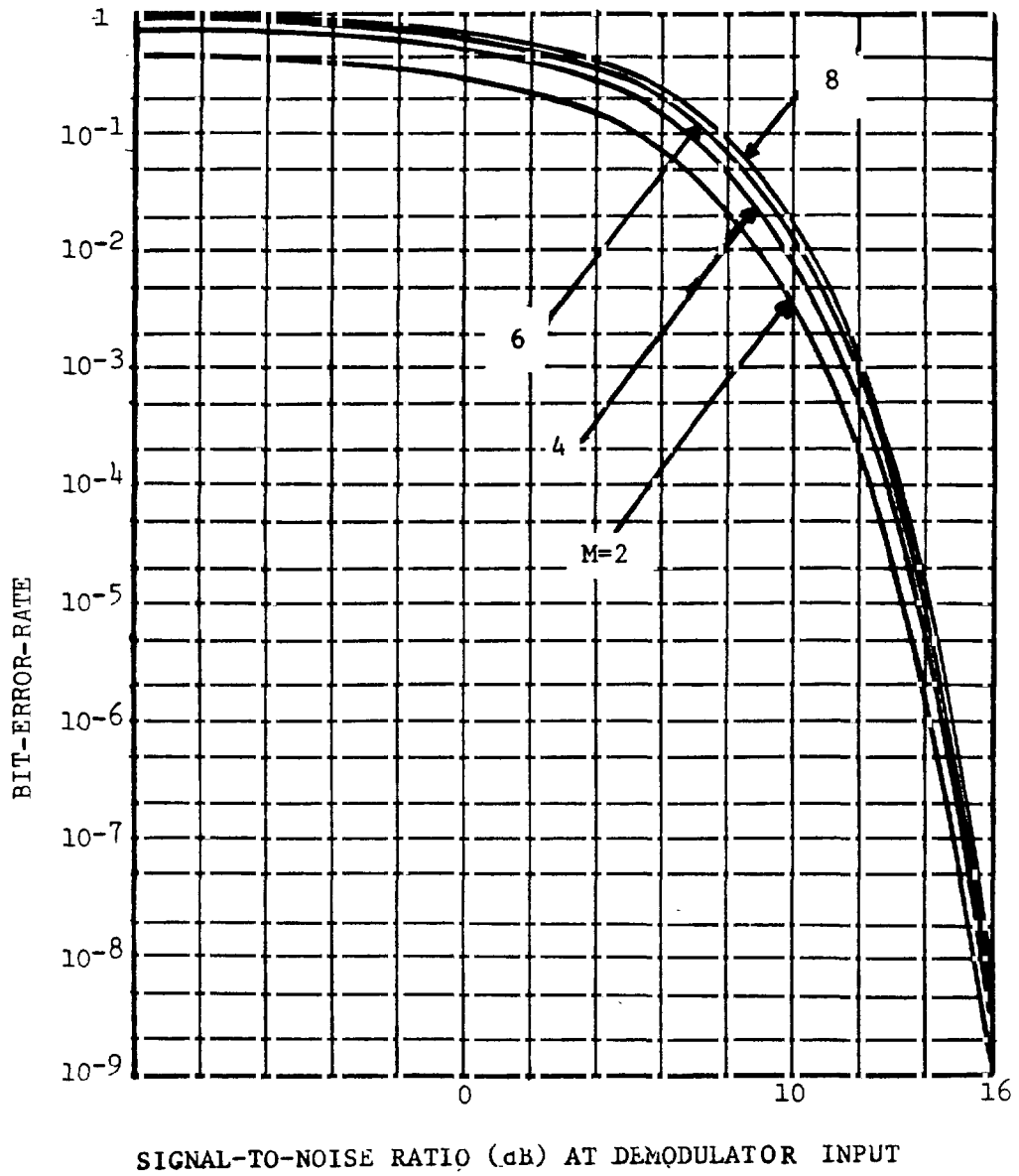
Figure 22. Probability of Bit-Error-Rate vs. Signal-to-Noise Ratio for FSK Modulation.
