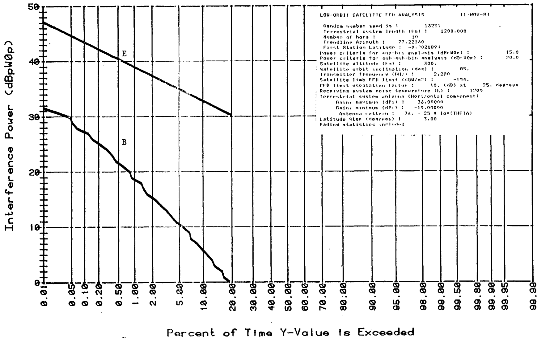
Figure 31 Interference Power from Eight Satellites in Non-Geostationary Orbits to Radio-Relay Receivers in a Trendline Using Frou Frequency Plan.
