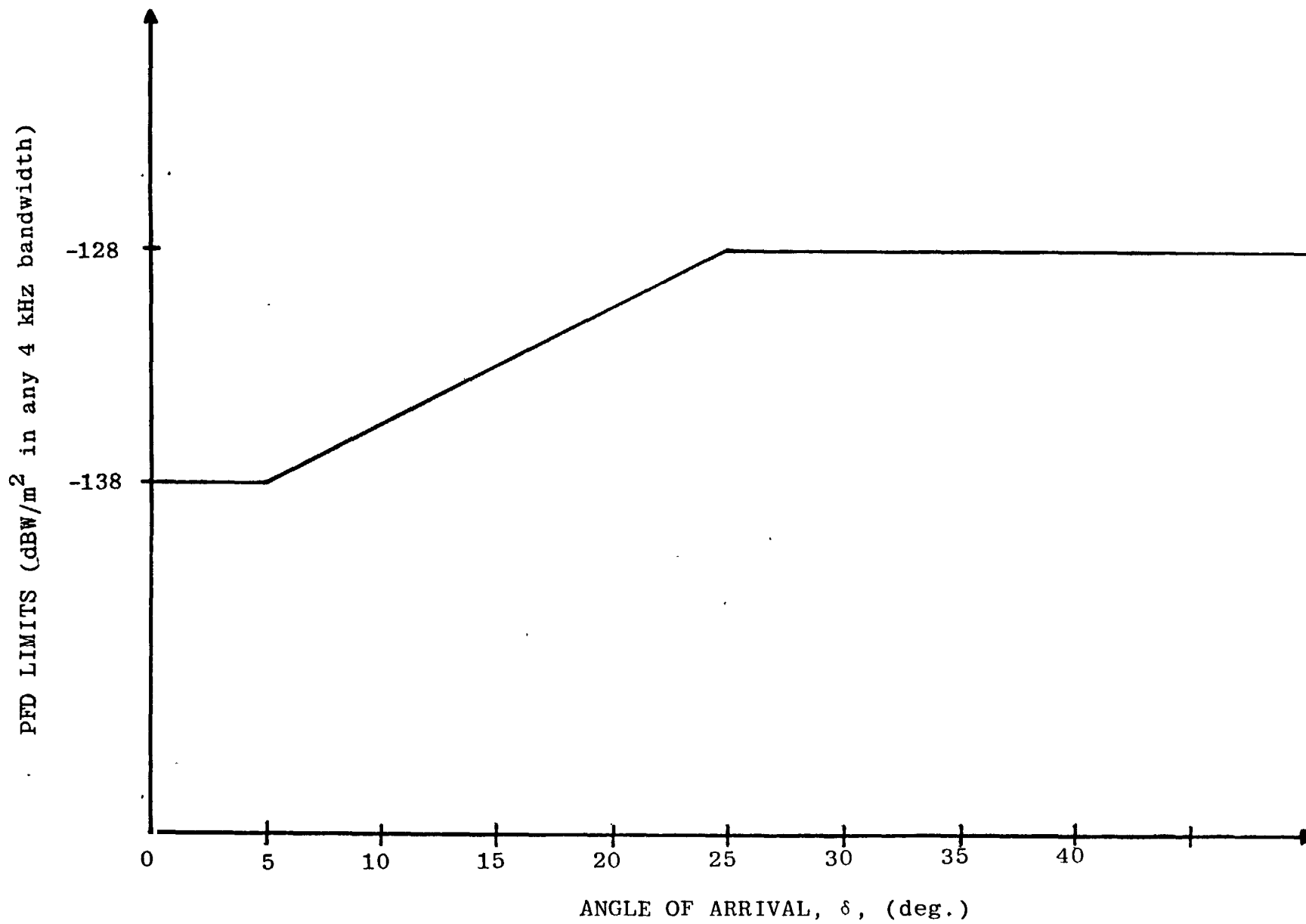
Figure 32 pfd Limits for Satellites in Non-Geostationary Orbits
