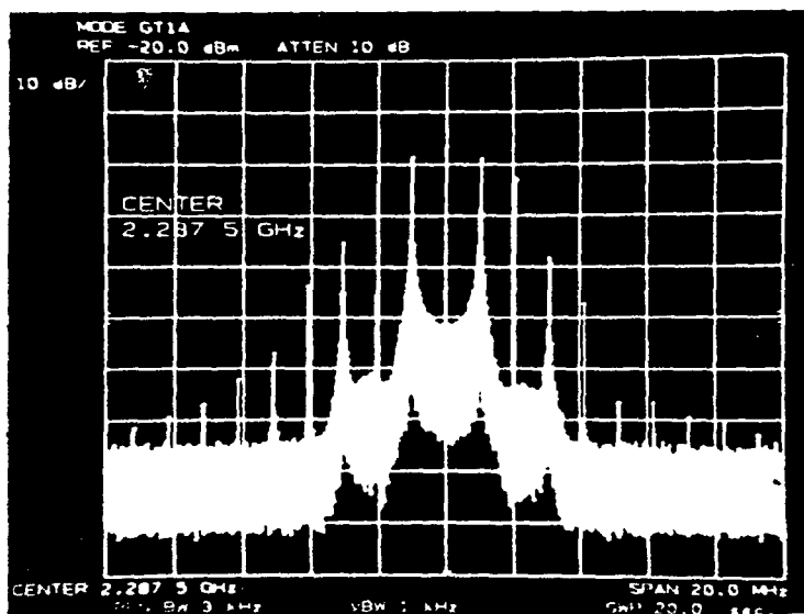
Figure 3 Mode GT1A emission from LANDSAT-D
