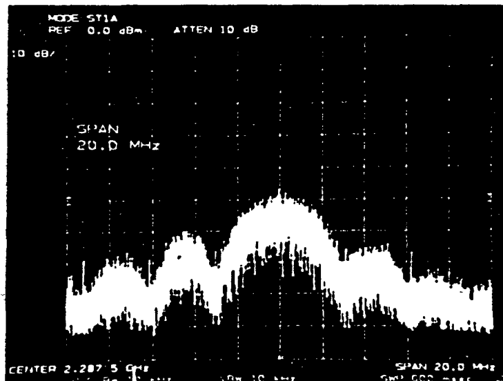
Figure 6 Emission spectrum of TDRSS down path transmission (\sin x/x)^2 .
