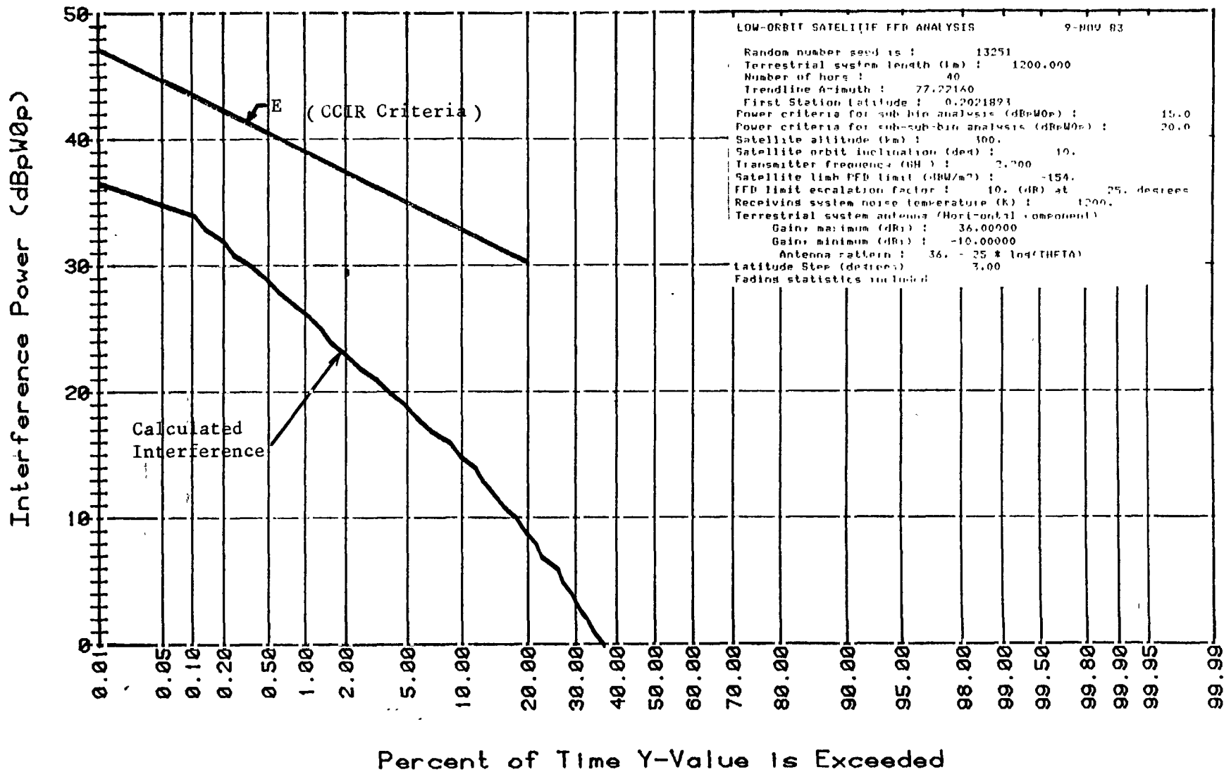
FIGURE 18: Interference from Satellites in Non-Geostationary Orbits.
