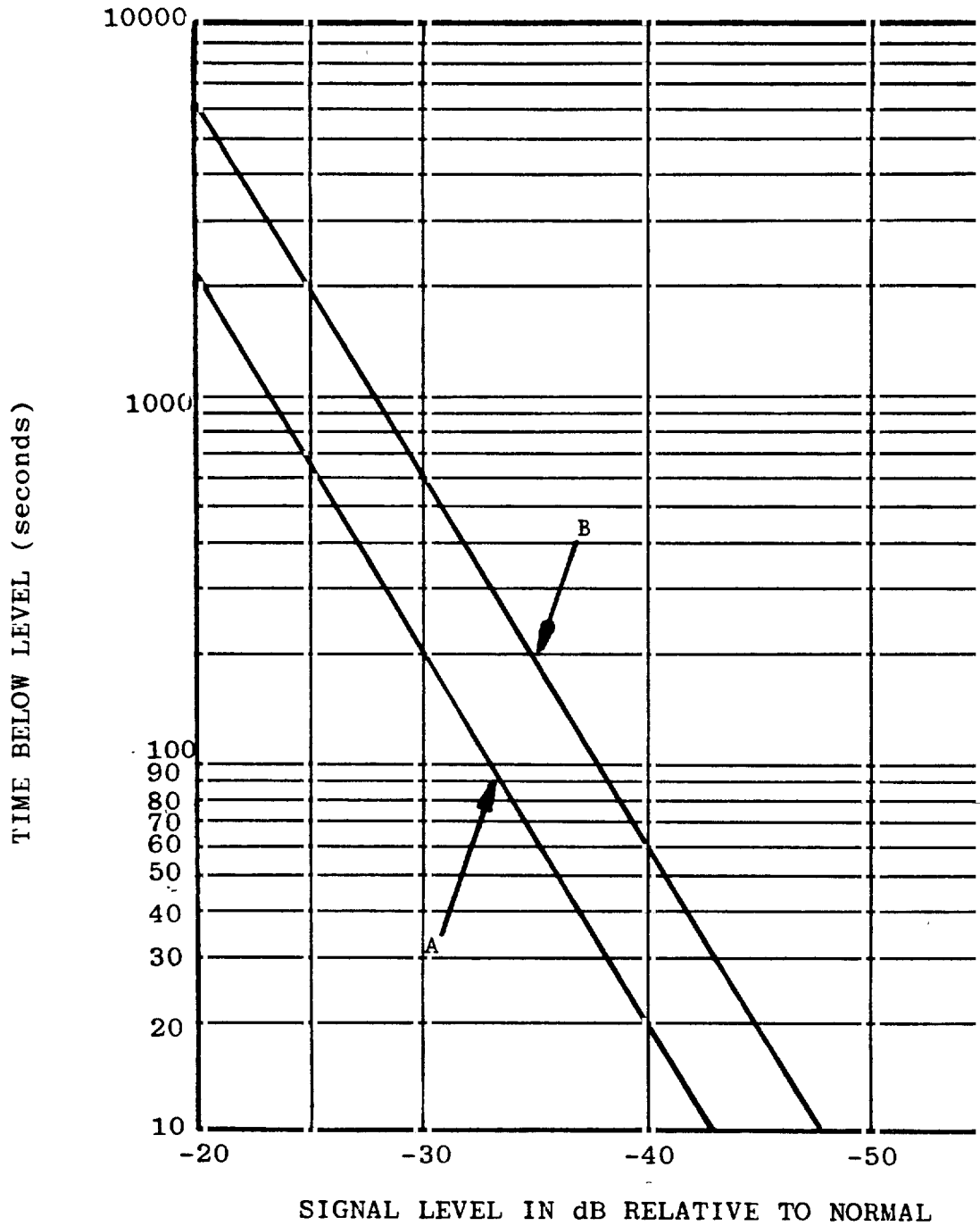
Figure 8 Time Below Level: A) Heavy Fading Month, B) Annual Fading (D=40 km, C=1, T_o=31 days = 2.68 \times 10^6 seconds).
