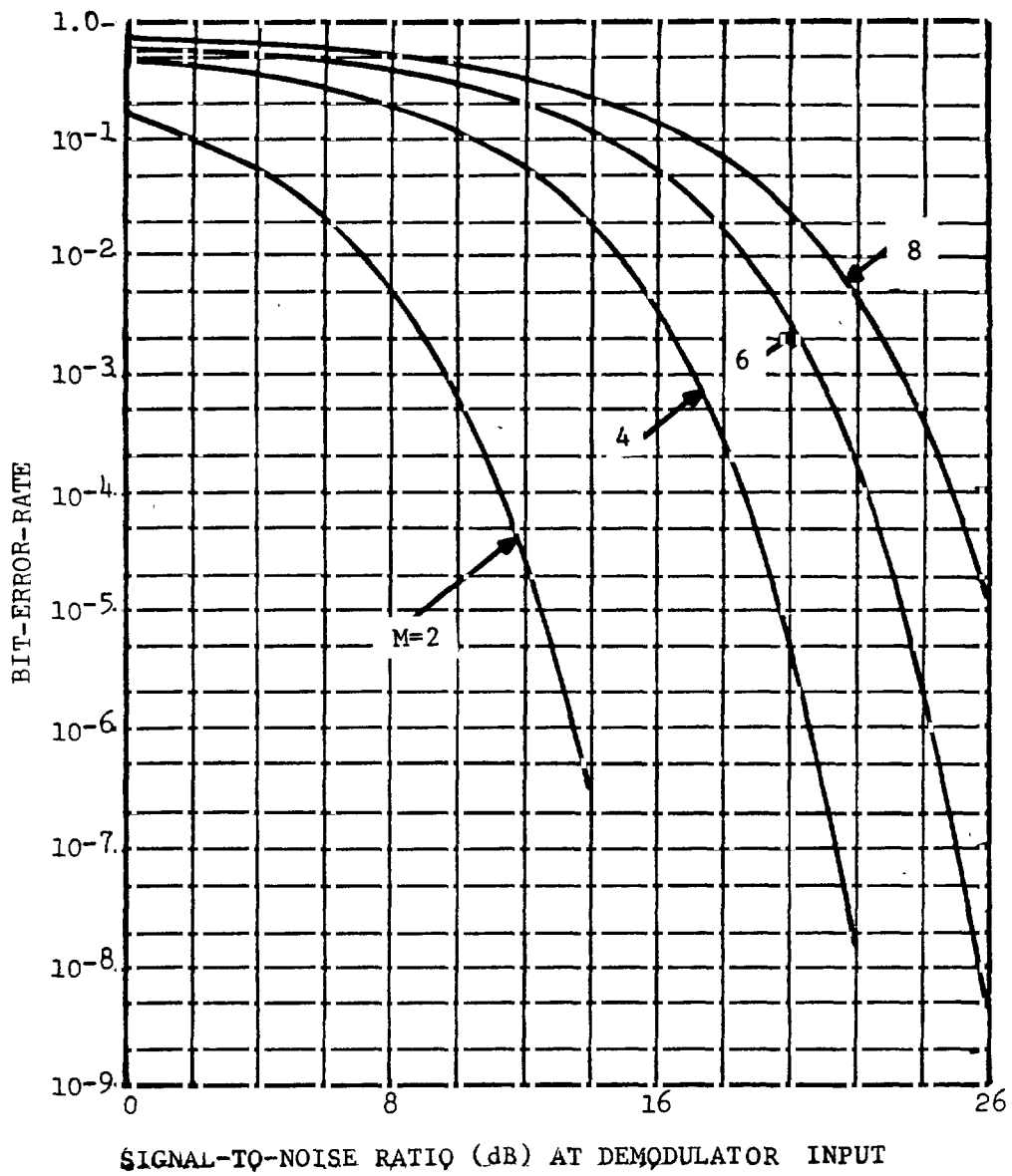
Figure 20. Probability of Bit-Error-Rate vs. Signal-to-Noise Ratio for ASK Modulation
