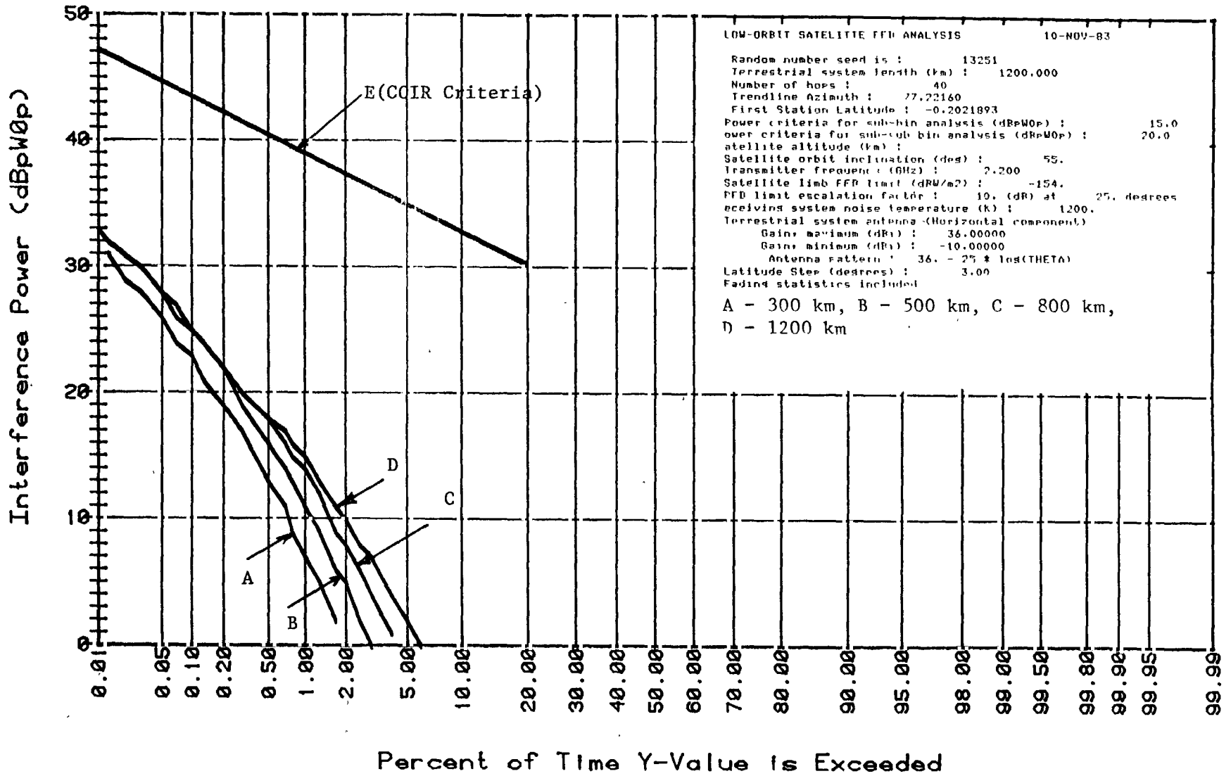
Figure 14 Interference Calculation for Inclination Angle Equal to 30 Degrees
