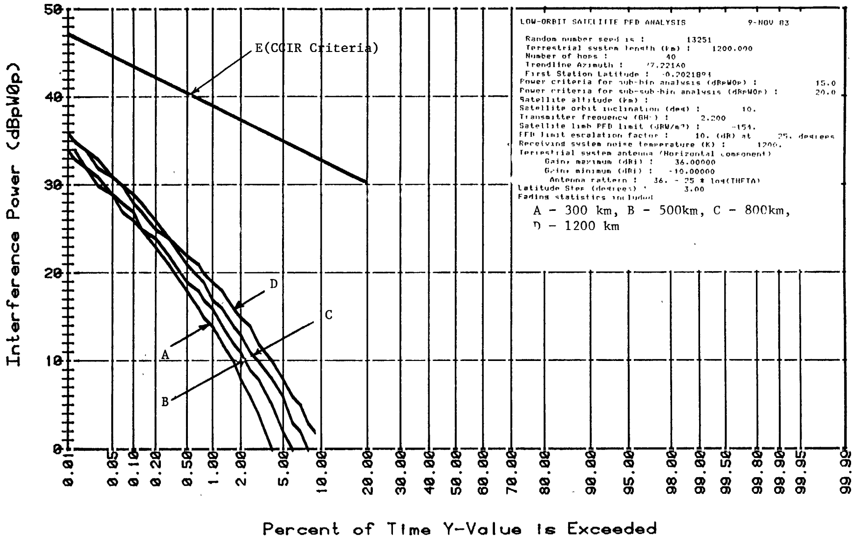
Figure 15 Interference Calculation for Inclination Angle Equal To 55 Degrees
