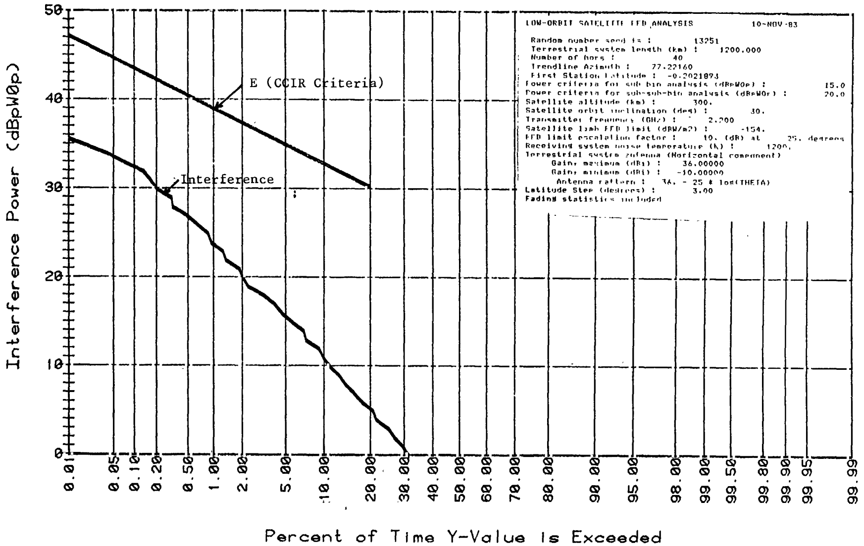
FIGURE 19: Interference Curve for 8 Satellites in Low Orbits Varying in Altitudes from 300-1200 km
