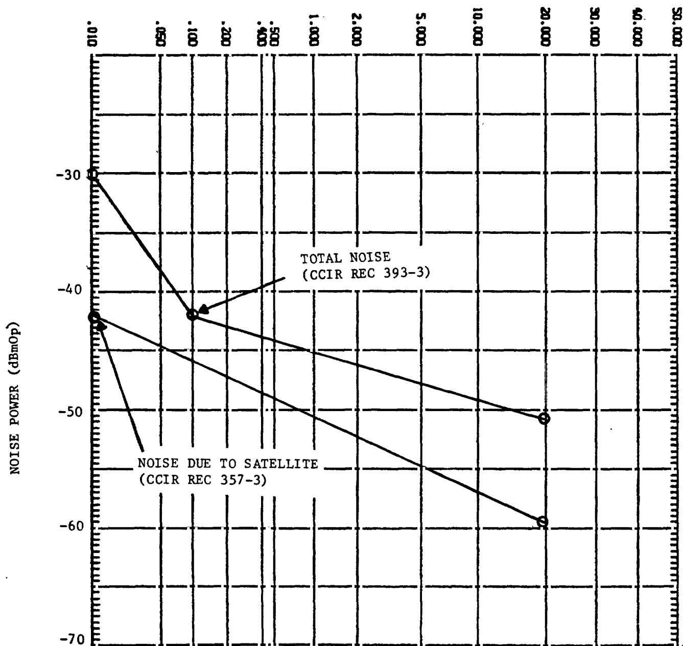
Figure 2. A Plot of CCIR Noise Power Level Criteria.
