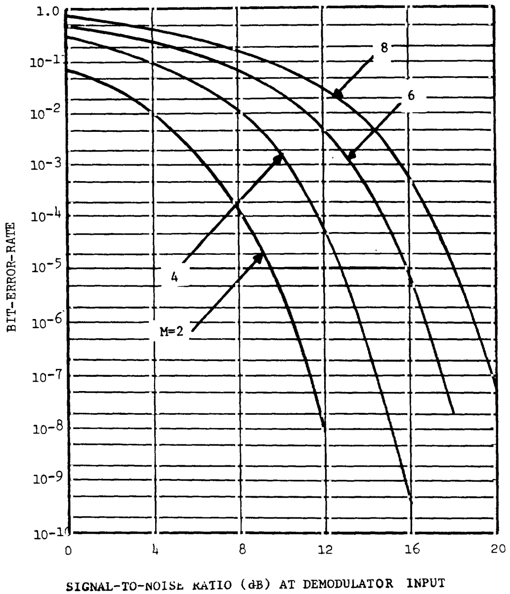
Figure 21. Probability of Bit-Error-Rate vs. Signal-to-Noise Ratio for PSK Modulation.
