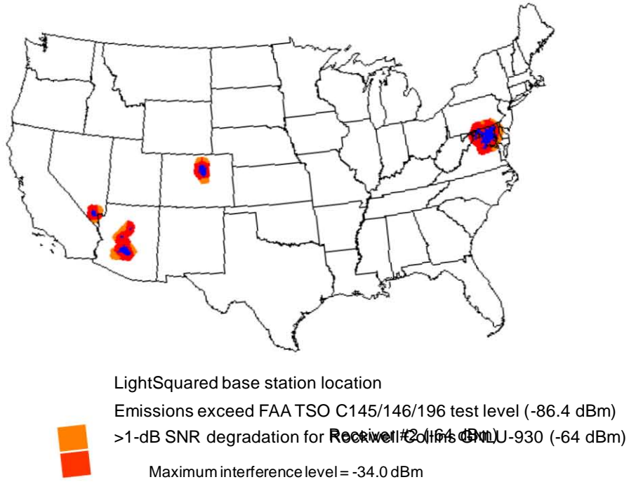
Figure 6-16. Initial LightSquared Deployment (2391 of 40000+ Towers) Aircraft at 200'
