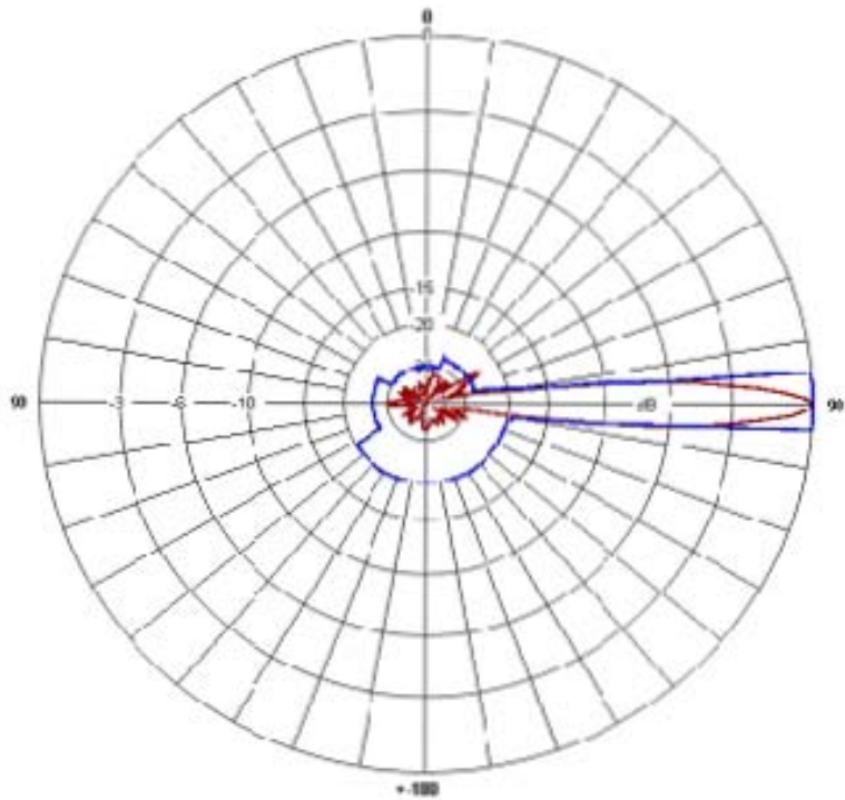
Relative Elev. Pattern (~7° beamwidth)
