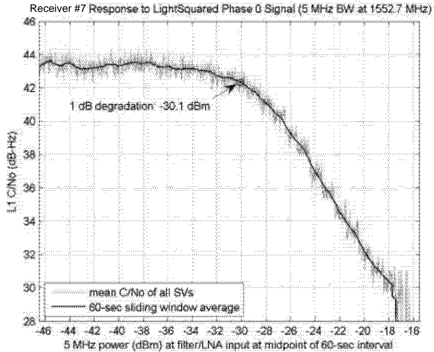
Figure 5-3. Receiver #7 C/N0 Response to LightSquared Phase 0 Signal
