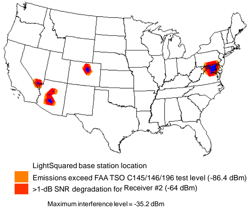
Figure 6-18. Initial LightSquared Deployment (2391 of 40000+ Towers) Aircraft at 350'
