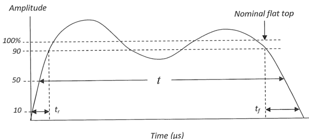
Figure 5.5.3.1b Schematic radar pulse diagrammed with cursors for rise time, fall time, and width
