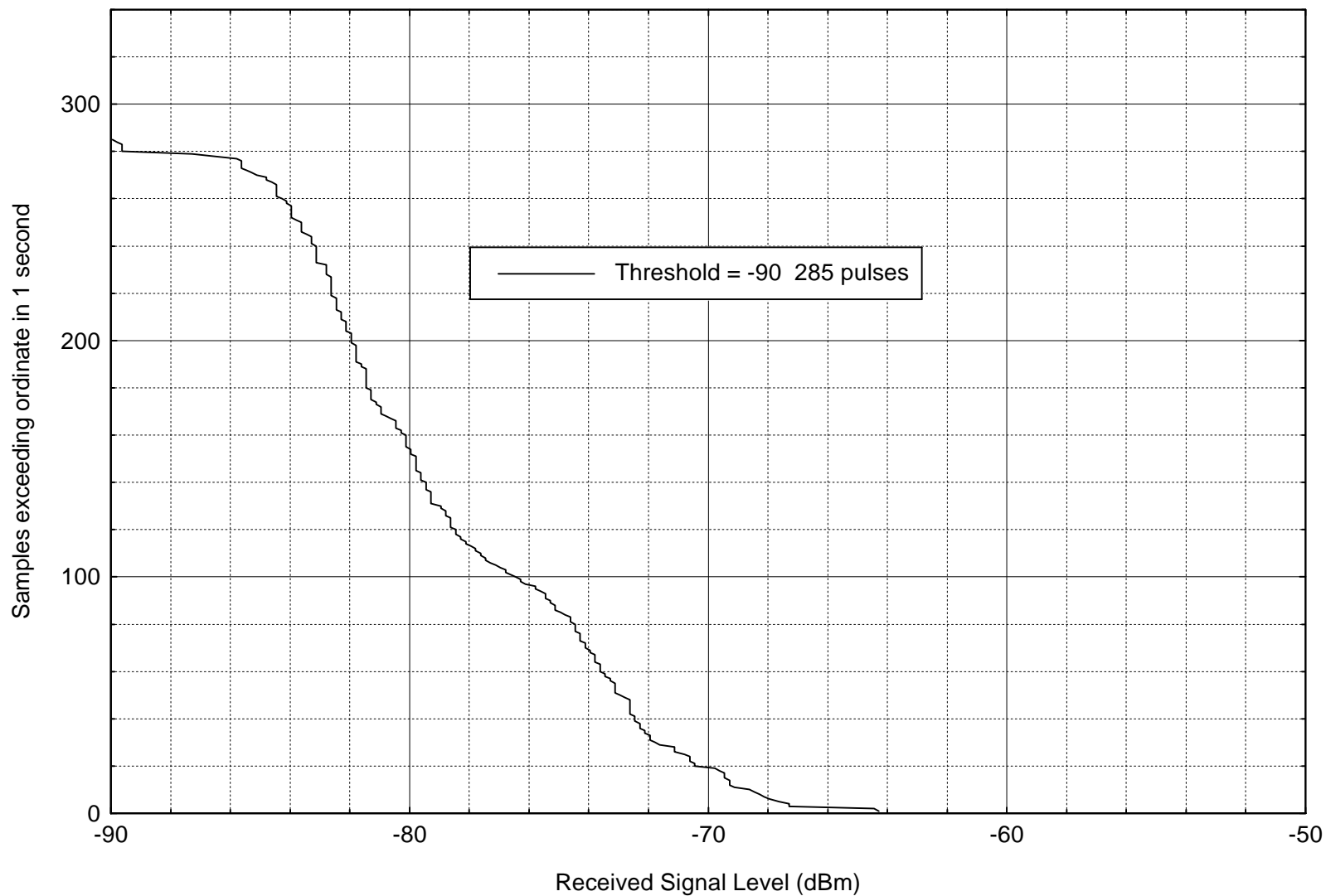
Figure 11. APD for direction to shipyard cranes, from earth station rooftop
