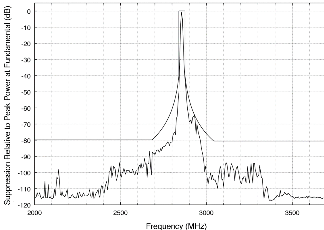
Figure 5-7 Criteria D Mask applied to radar emissions
