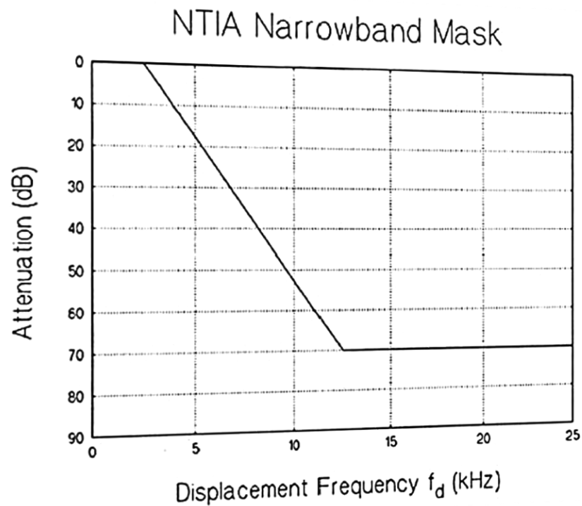
Figure 5.3.7.1 Levels of Unwanted Emissions
