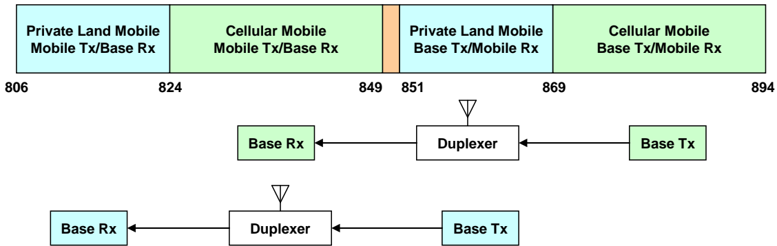
Figure 9 – Duplex scenarios in the 800 MHz band.
