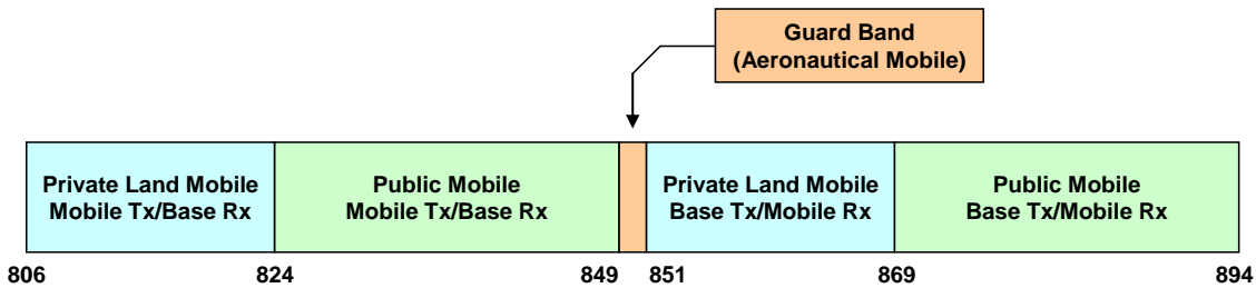
Figure 8 – The 800 MHz land mobile band and associated guardband
