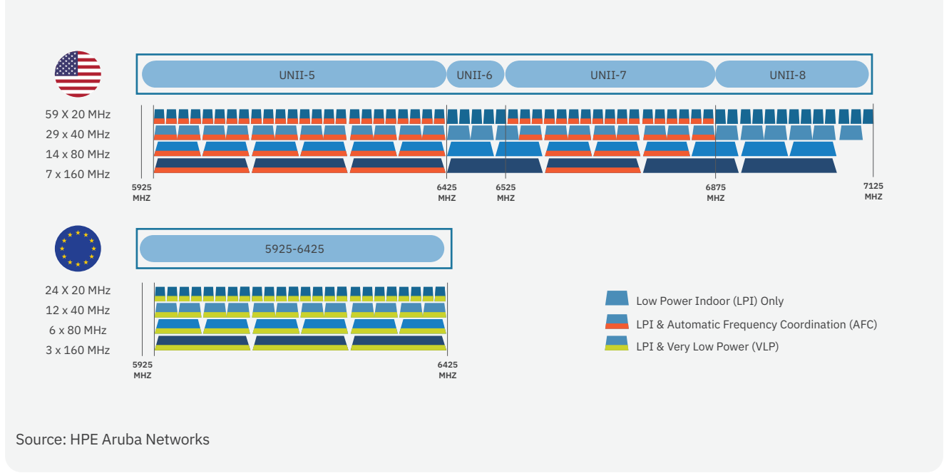
Figure 14: Available 6 GHz channels for Wi-Fi 6E in Europe versus the US
