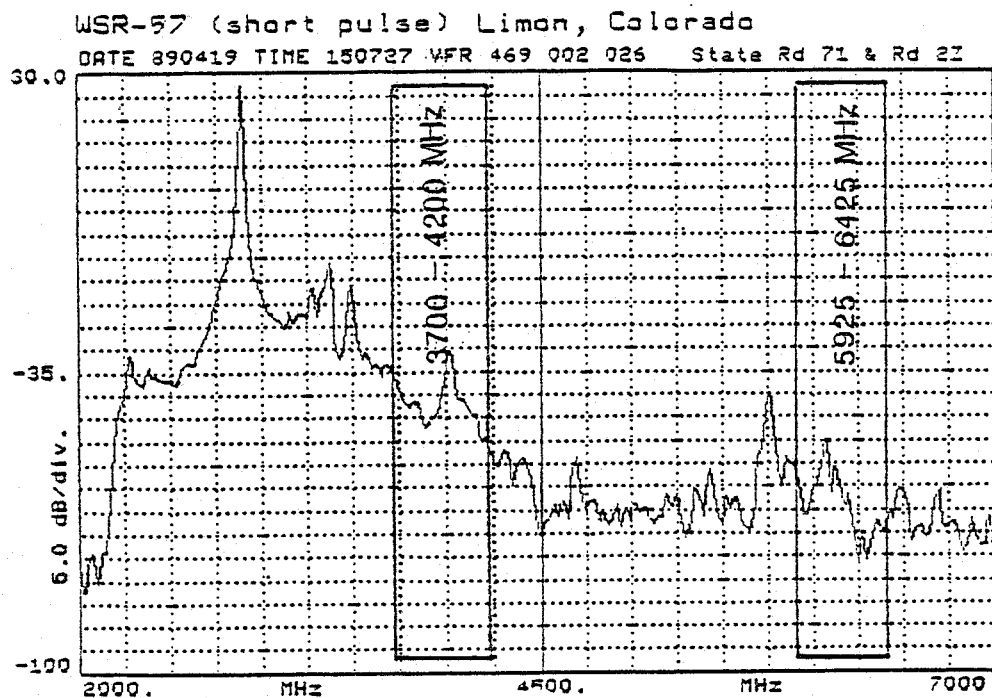
Figure 5-14. Radiated spectrum measurements of spurious emission levels for the WSR-57 conventional magnetron with a short pulse (measured with 30 MHz bandwidth).
