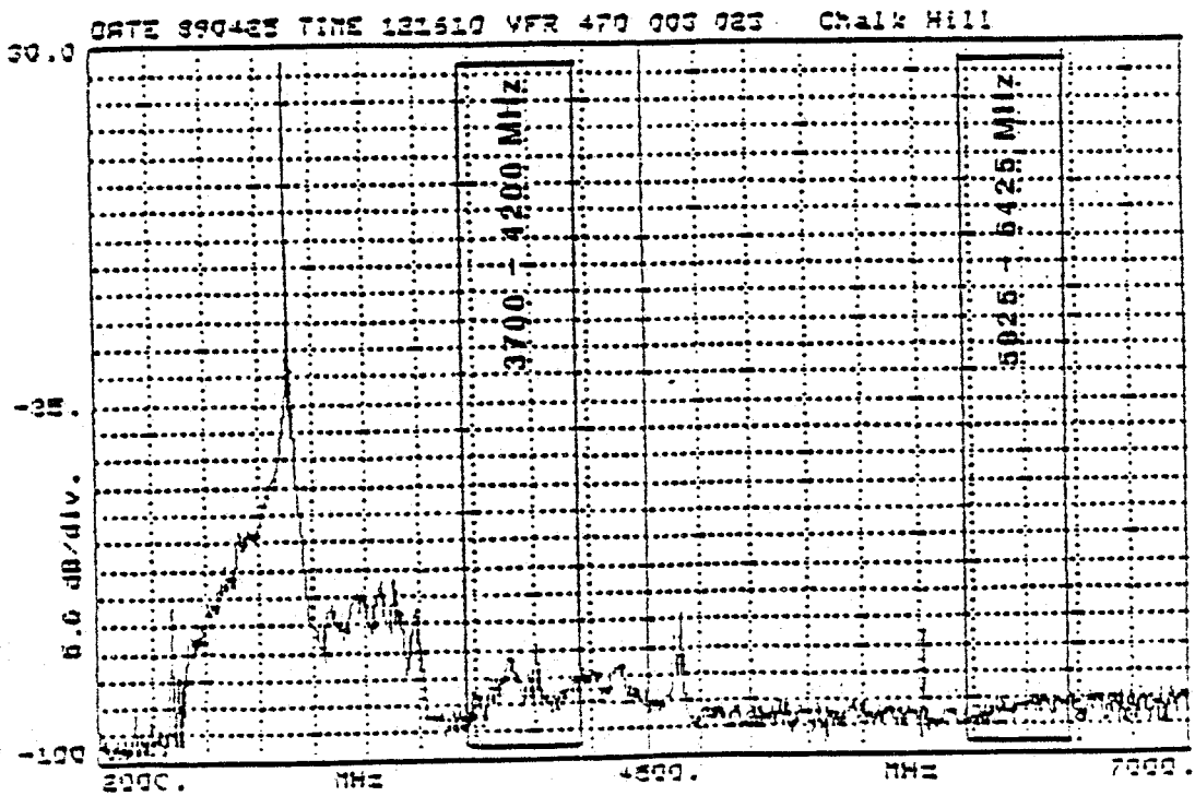
Figure 5-6. Radiated spectrum measurements of the WSR-74S radar at Longview, TX (pulsewidth = 1 \mu s).
