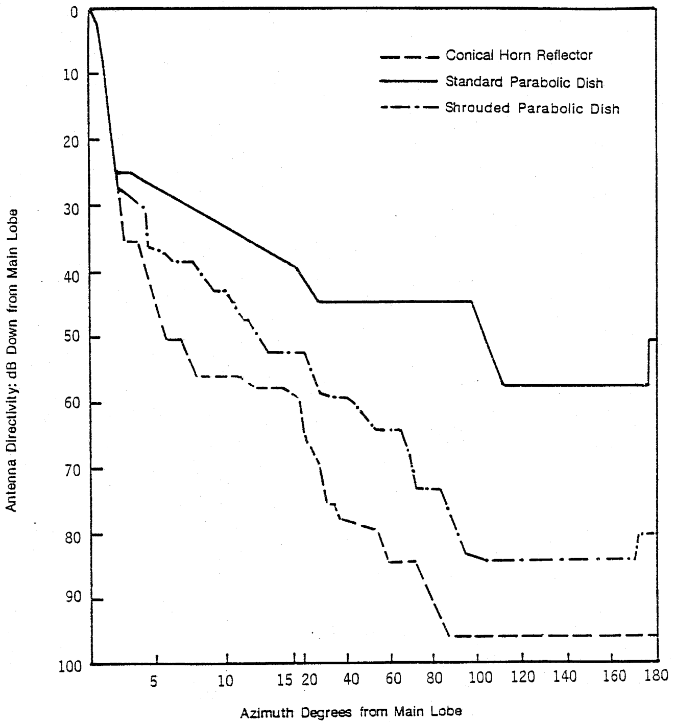
Figure 6-1. Comparison of typical 10 foot (3 m) 4/6 GHz Common Carrier Radio Relay Antennas.
