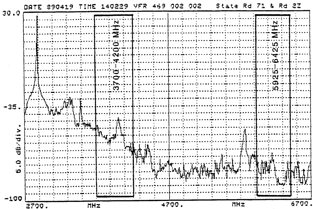
Figure 5-2. Radiated spectrum measurements of the WSR-57 radar at Limon, CO, (pulsewidth = 4 \mu s).
