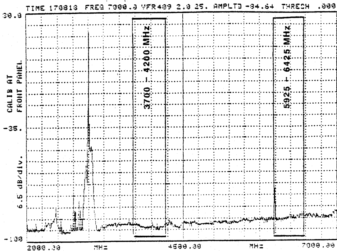
Figure 5-12. Radiated spectrum measurements of the test and evaluation NEXRAD radar at Norman, OK, (pulswidth = 1.67 \mu s).
