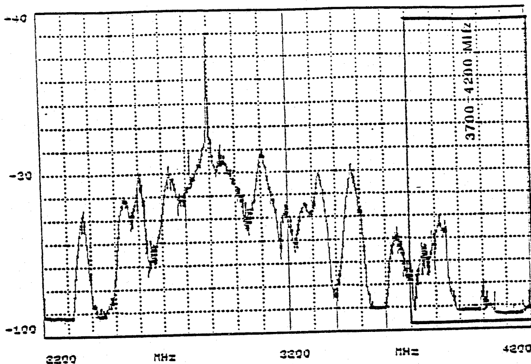
Figure 5-3. Radiated spectrum measurements of the WSR-74S radar at Portland, ME, (pulsewidth = 4 \mu s).
