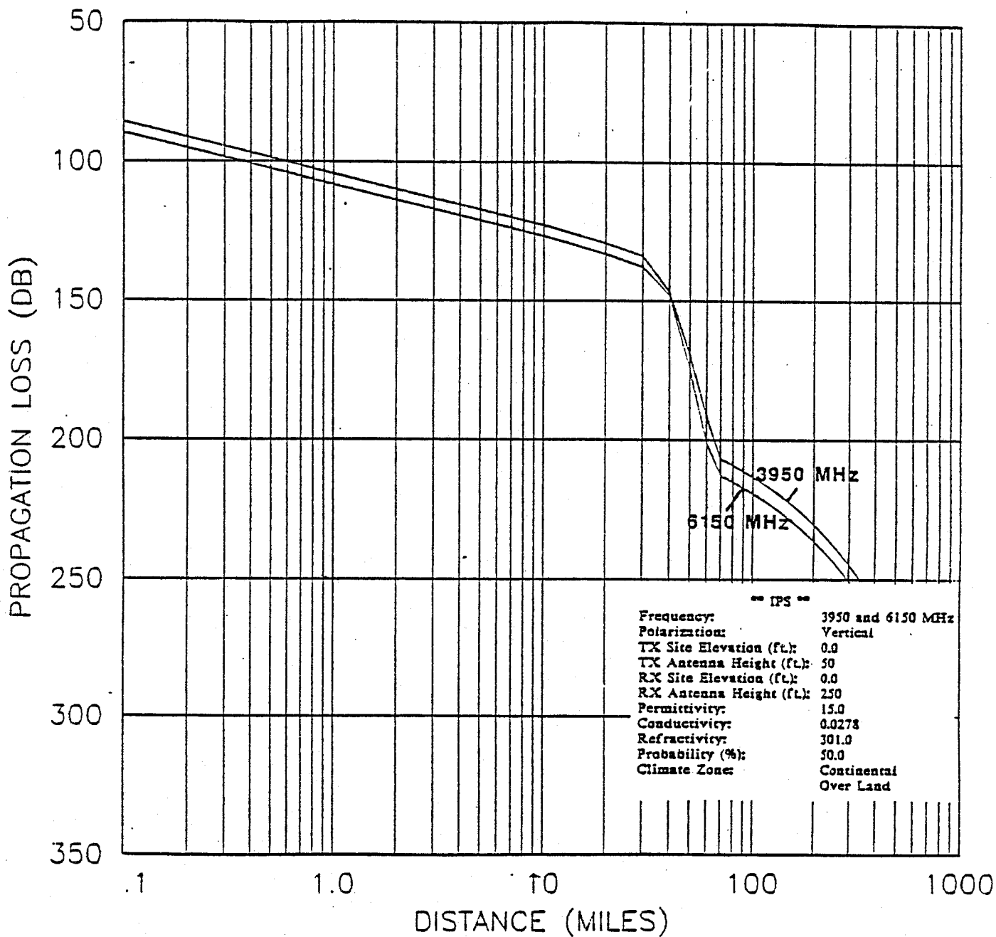
Figure 5-22. Propagation Loss versus Distance Separation curves.
