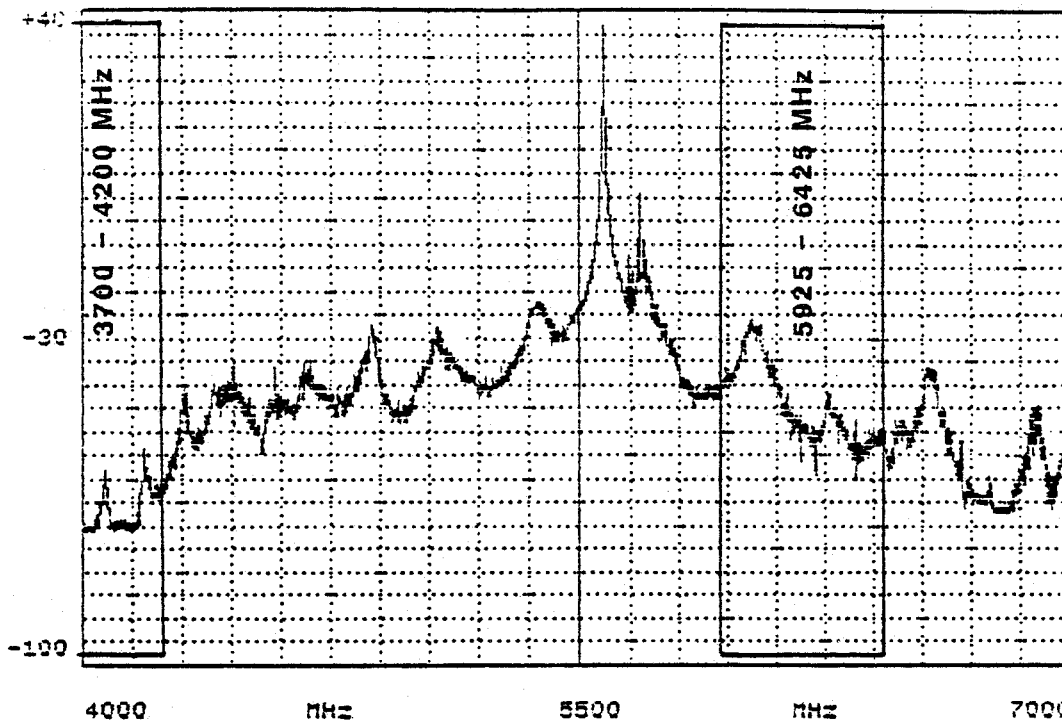
Figure 5-9. Radiated spectrum measurements of the WR100-2 radar at Golden, CO (pulsewidth = 3 \mu s).
