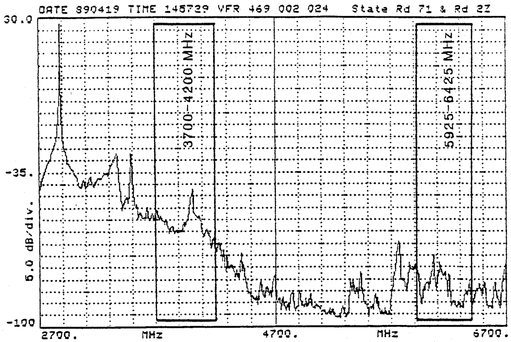
Figure 5-1. Radiated spectrum measurements of the WSR-57 radar at Limon, CO, (pulsewidth = 1 \mu s).
