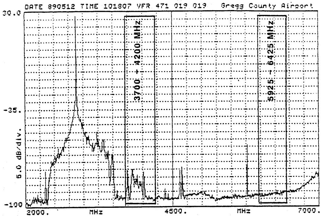
Figure 5-7. Radiated spectrum measurements of the WSR-74S radar at Longview, TX (pulsewidth = 4 \mu s).
