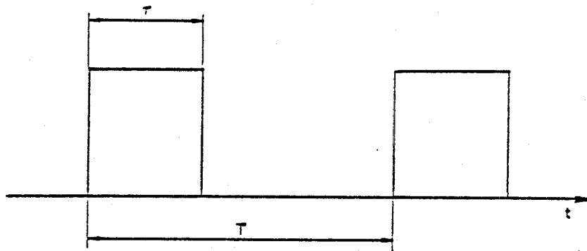
Figure E-1. Input radar pulse time waveform.
