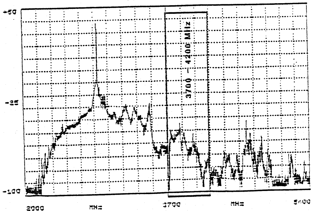
Figure 5-4. Radiated spectrum measurements of the WSR-74S radar at Volens, VA (pulsewidth = 1 \mu s).
