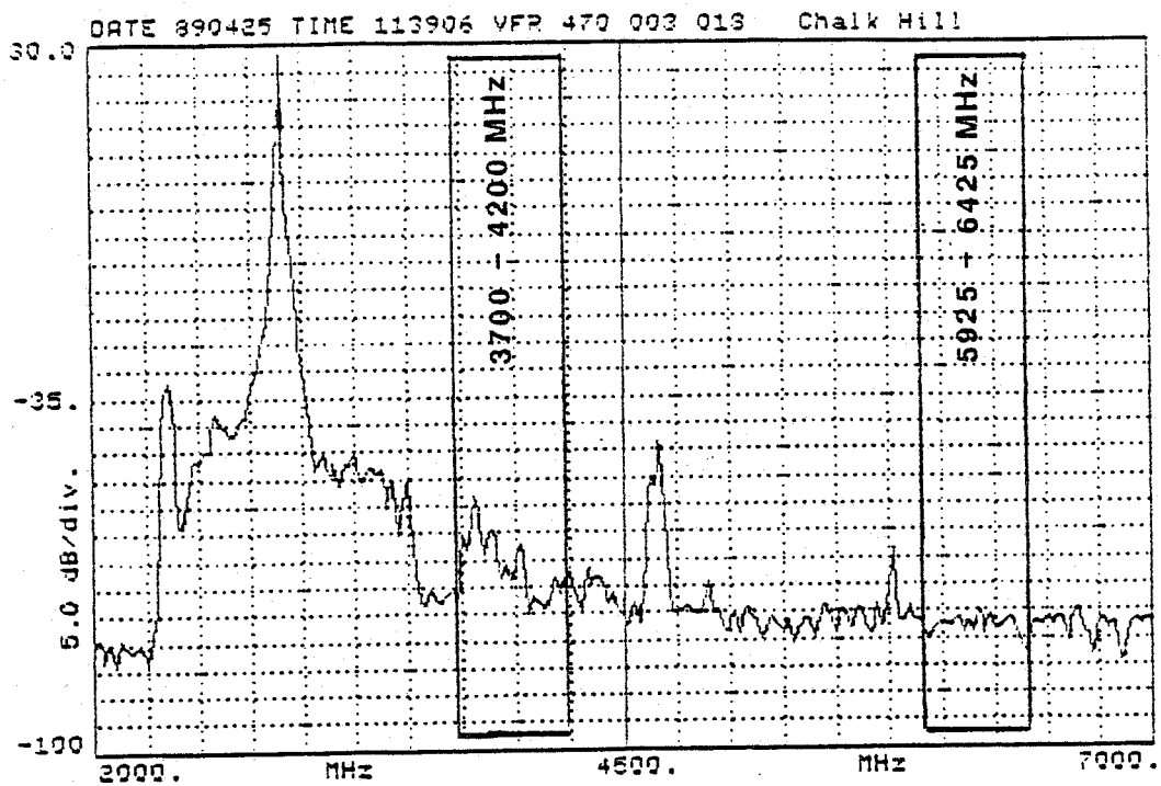
Figure 5-17. Radiated spectrum measurements of spurious emission levels for the WSR-74S coaxial magnetron with a long pulse (measured with 30 MHz bandwidth).
