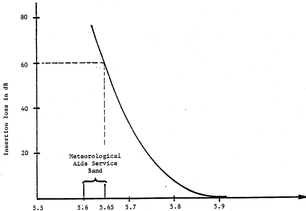
Figure B-2. Insertion loss versus frequency for a waveguide filter used to block meteorological radar.
