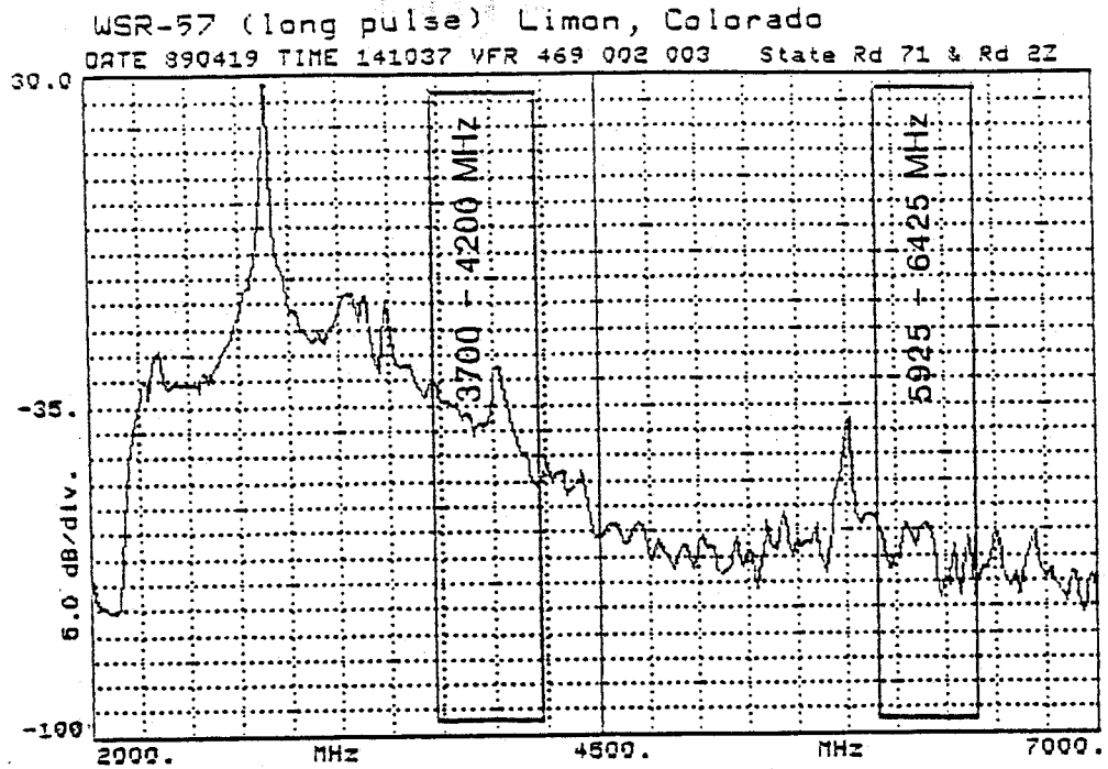
Figure 5-15. Radiated spectrum measurements of spurious emission levels for the WSR-57 conventional magnetron with a long pulse (measured with 30 MHz bandwidth).
