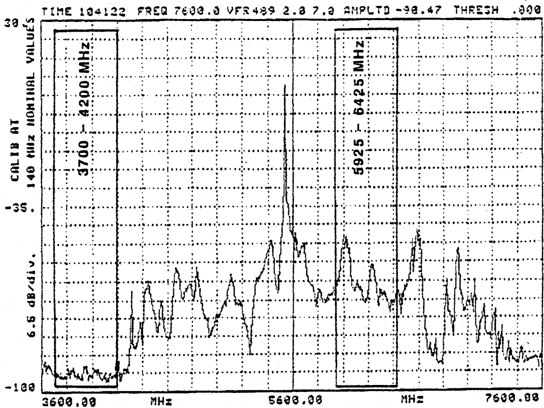
Figure 5-11. Radiated spectrum measurements of the DWSR-88 CTV radar at Tulsa, OK (pulswidth 0.8 \mu s).
