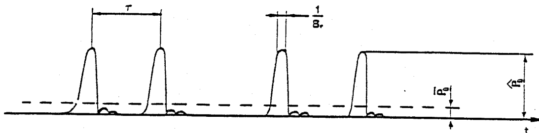
Figure E-2. Output time waveform for condition B_r > 1/T and large frequency deviation ( \Delta f ) from the tuned frequency.
