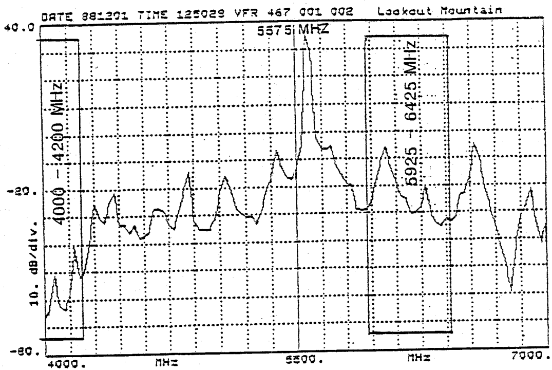
Figure 5-18. Radiated spectrum measurements of spurious emission levels for the WR100-2 coaxial magnetron (measured with 30 MHz bandwidth).
