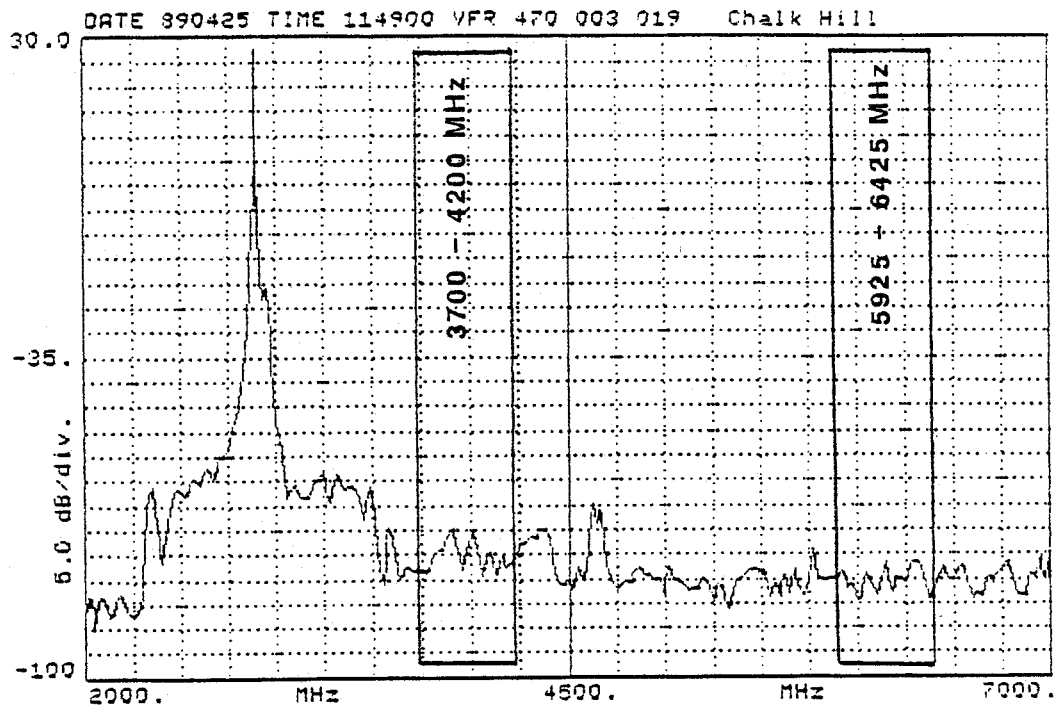
Figure 5-16. Radiated spectrum measurements of spurious emission levels for the WSR-74S coaxial magnetron with a short pulse (measured with 30 MHz bandwidth).
