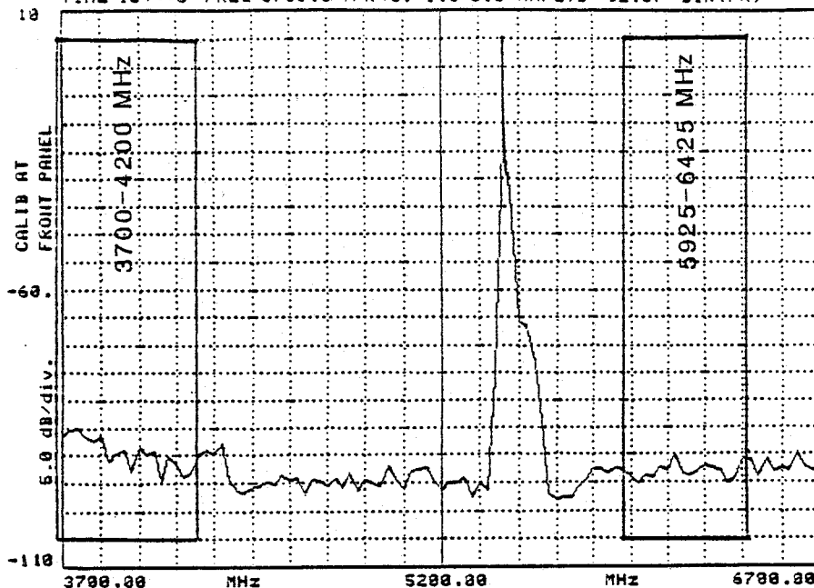
Figure 5-13. Radiated spectrum measurements of the WRT-710C radar at Denver, CO.
