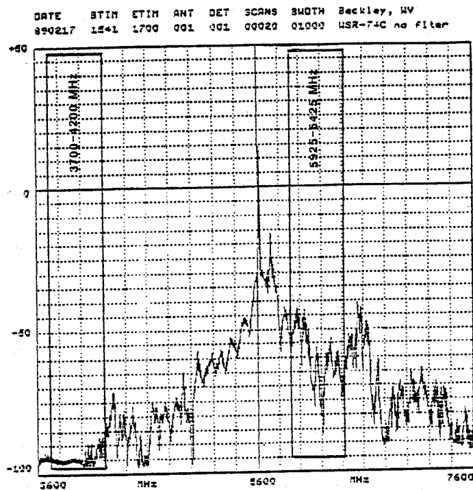
Figure 5-8. Radiated spectrum measurements of the WSR-74C radar at Beckley, WV (pulsewidth = 3 \mu s).
