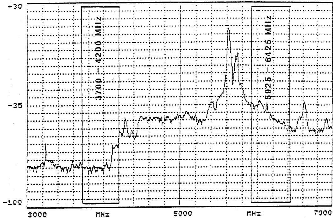
Figure 5-19. Radiated spectrum measurements of spurious emission levels for the WSR-74C coaxial magnetron (measured with 30 MHz bandwidth).
