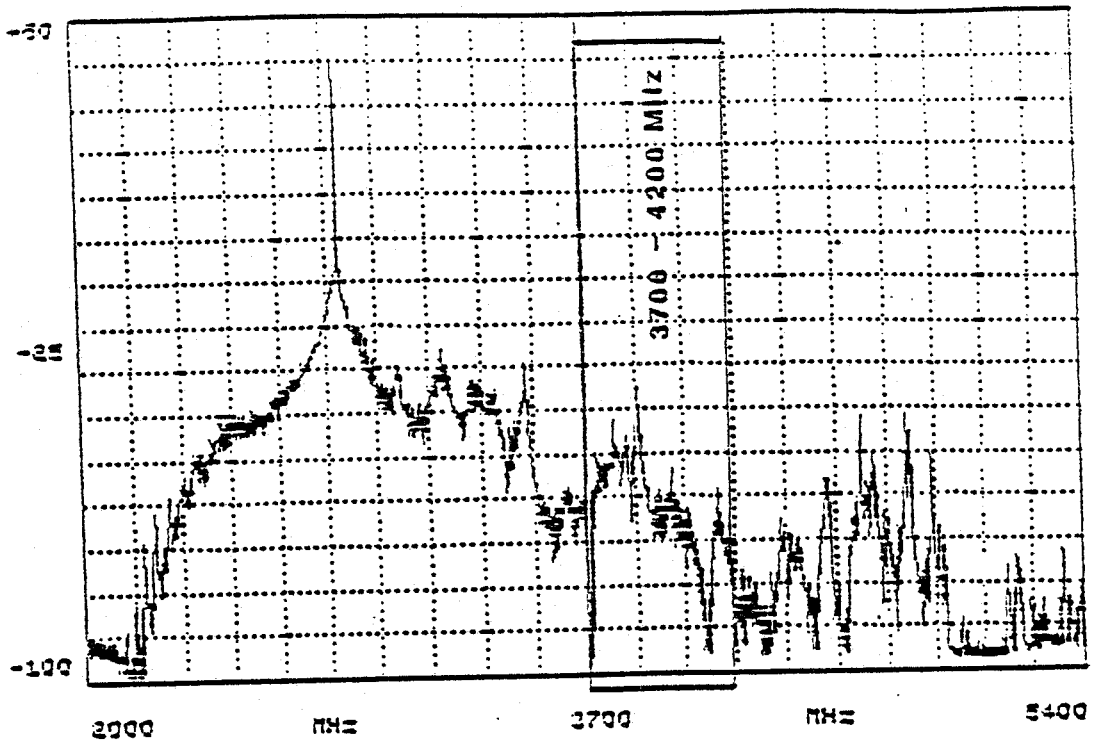
Figure 5-5. Radiated spectrum measurements of the WSR-74S radar at Volens, VA (pulsewidth = 4 \mu s).
