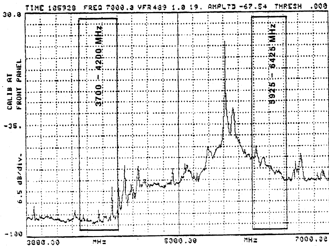
Figure 5-10. Radiated spectrum measurements of WSR-74C radar at Tulsa, OK (pulsewidth = 3.0 \mu s).
