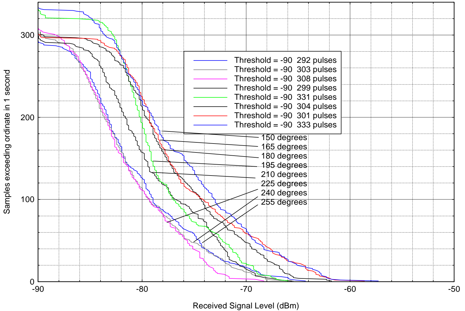
Figure 9. APDs for 150-255 degrees azimuth, on earth station rooftop
