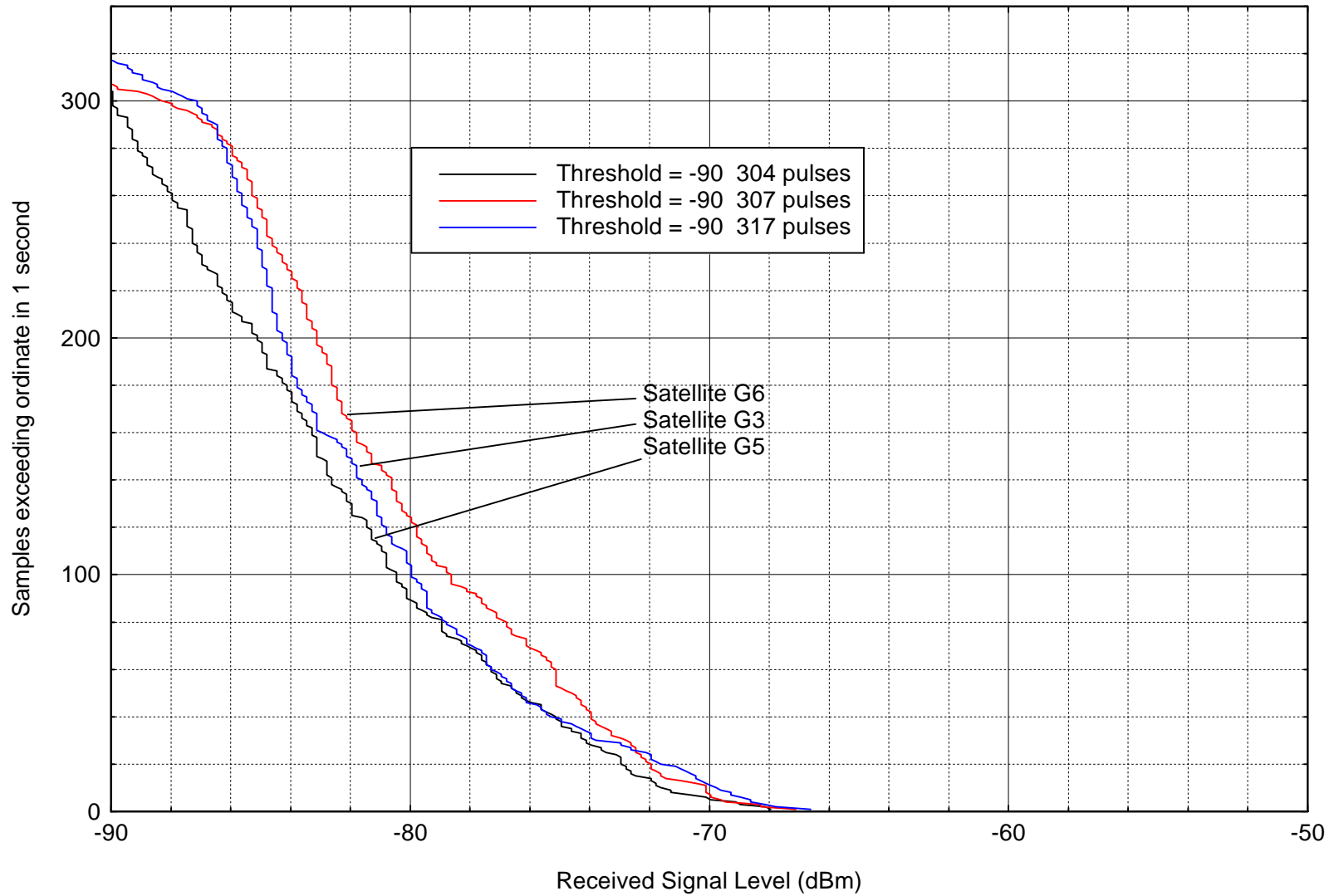
Figure 10. APDs for line-of-sight of earth station antennas, from rooftop
